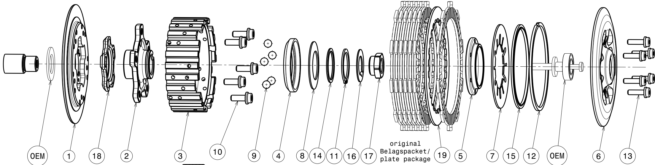
Partlist: 2064
