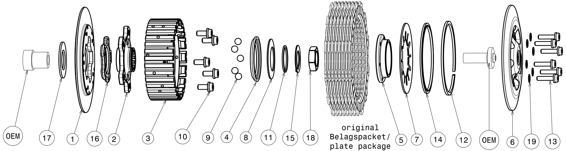
Partlist: 2521
